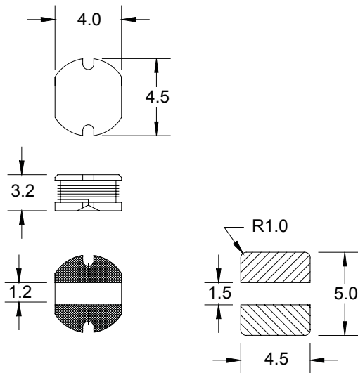
Dimensions: mm Tolerance: -/+0.3
